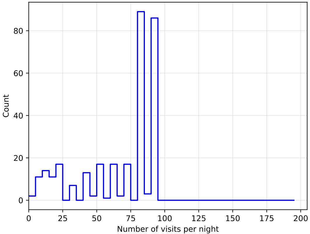
mw_roll_all_v3.3_10yrs all bands: DD:ECDFS NVisitsPerNight
