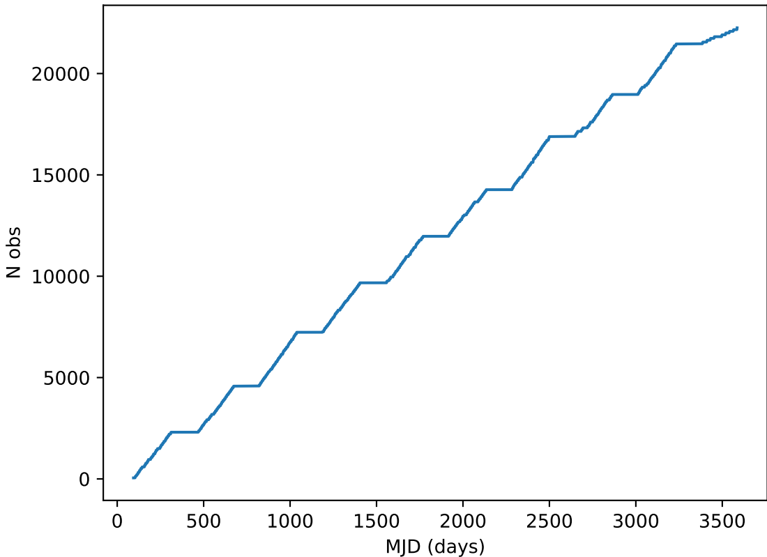
mw_roll_all_v3.3_10yrs all bands: DD:ECDFS Cumulative NVisits
