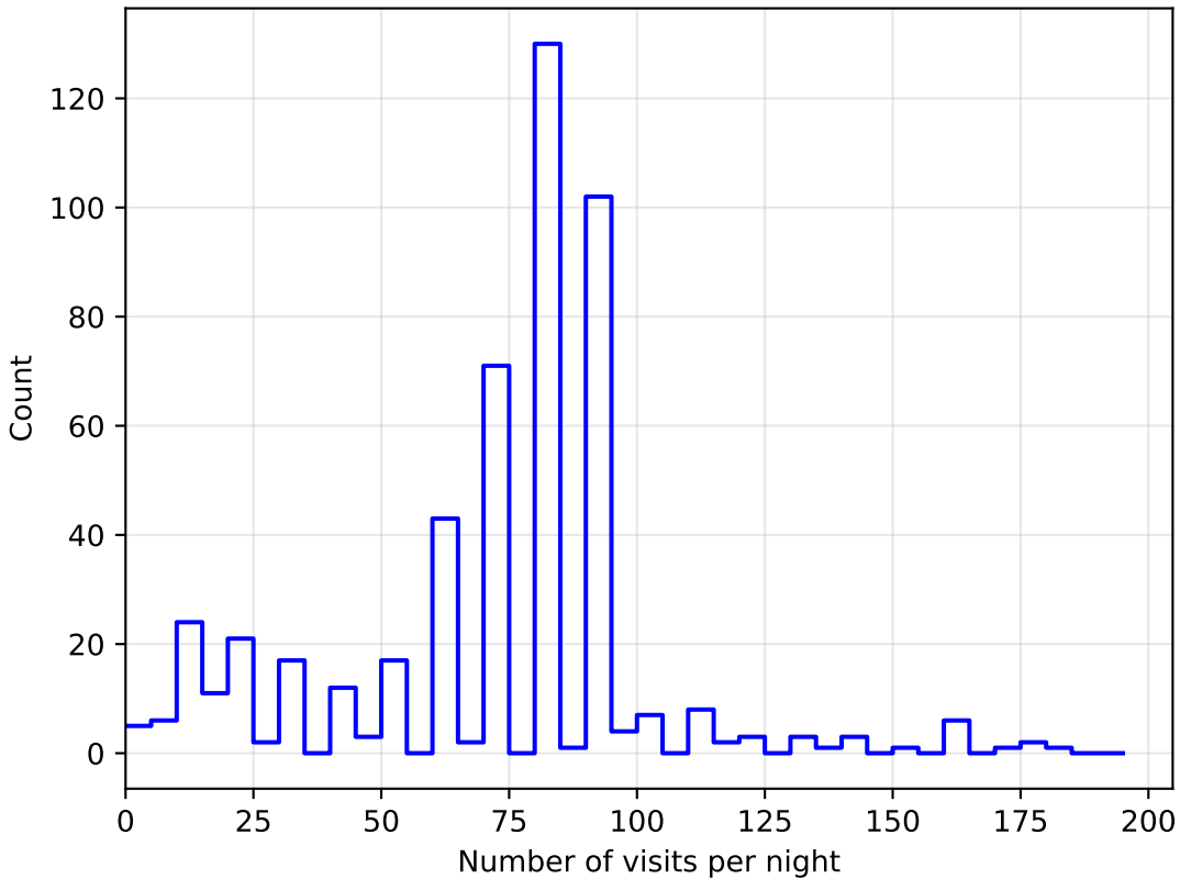
mw_roll_all_v3.3_10yrs all bands: DD:COSMOS NVisitsPerNight
