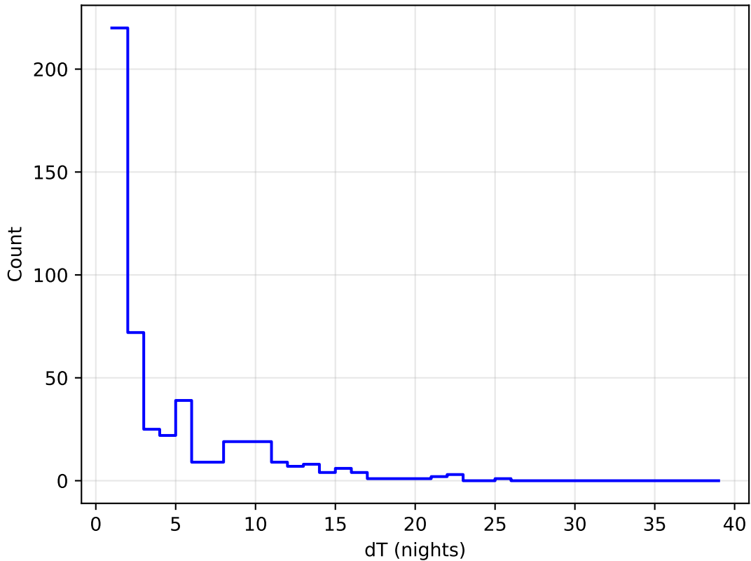
mw_roll_all_v3.3_10yrs all bands: DD:COSMOS Delta Nights Histogram
