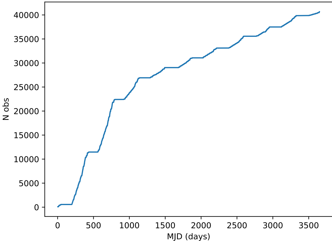
mw_roll_all_v3.3_10yrs all bands: DD:COSMOS Cumulative NVisits
