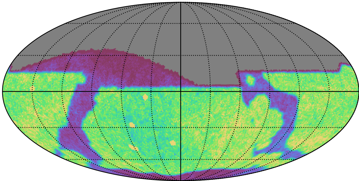
lmc_filter_balance_v3.4_10yrs night < 365.25: Year1.0Count
