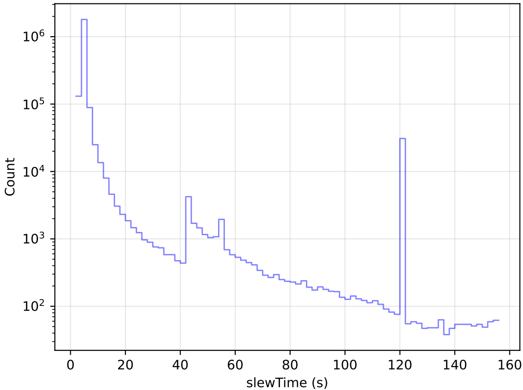
Imc_filter_balance_v3.4_10yrs All visits: Slew Time Histogram
