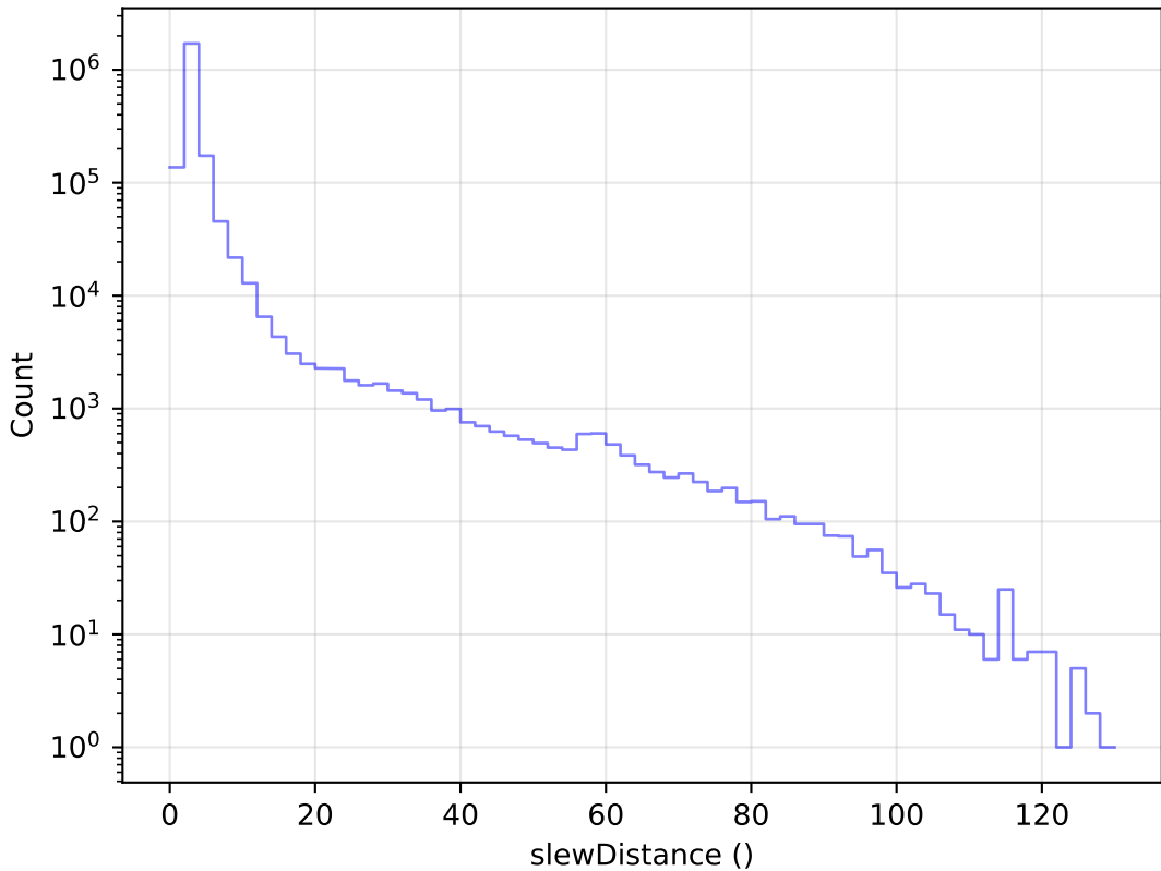
Imc_filter_balance_v3.4_10yrs All visits: Slew Distance Histogram
