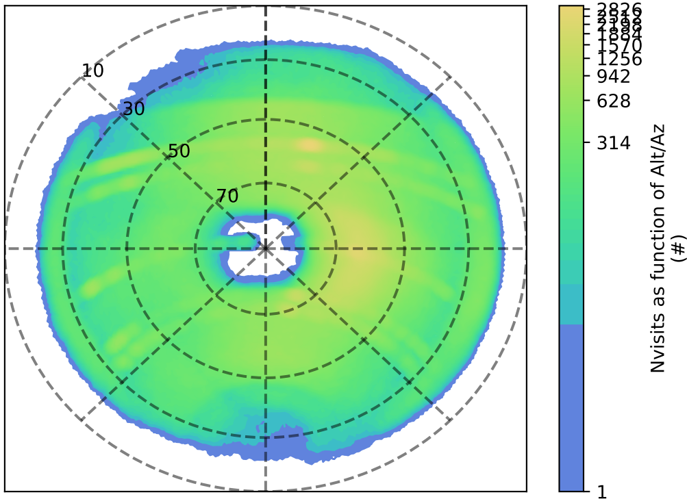
lmc_filter_balance_v3.4_10yrs z: Nvisits as function of Alt/Az
