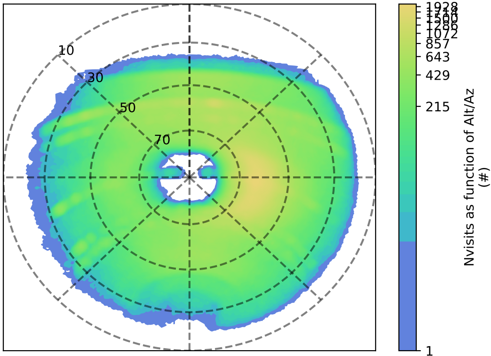
lmc_filter_balance_v3.4_10yrs y: Nvisits as function of Alt/Az
