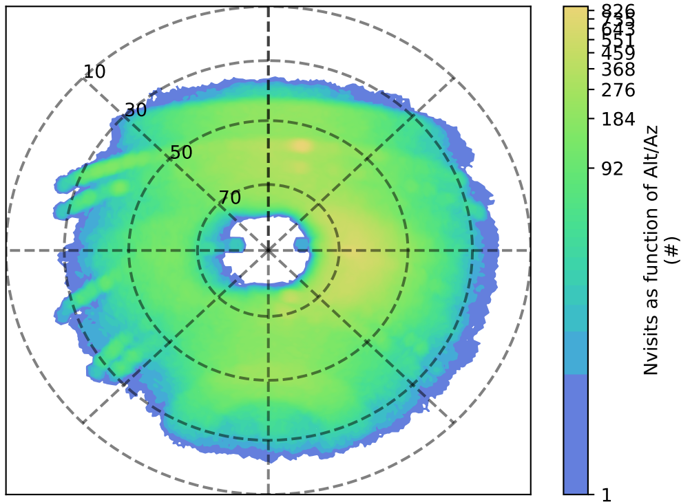
lmc_filter_balance_v3.4_10yrs u: Nvisits as function of Alt/Az
