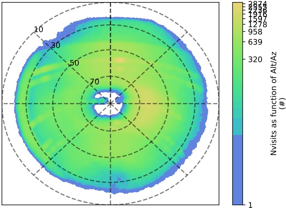
lmc_filter_balance_v3.4_10yrs r: Nvisits as function of Alt/Az
