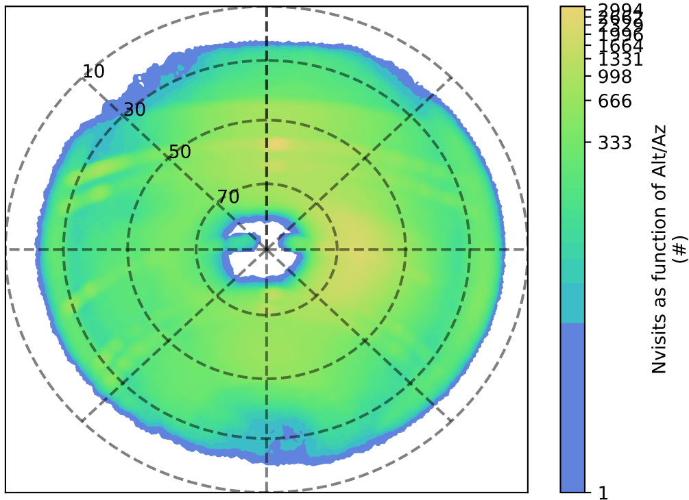
lmc_filter_balance_v3.4_10yrs i: Nvisits as function of Alt/Az
