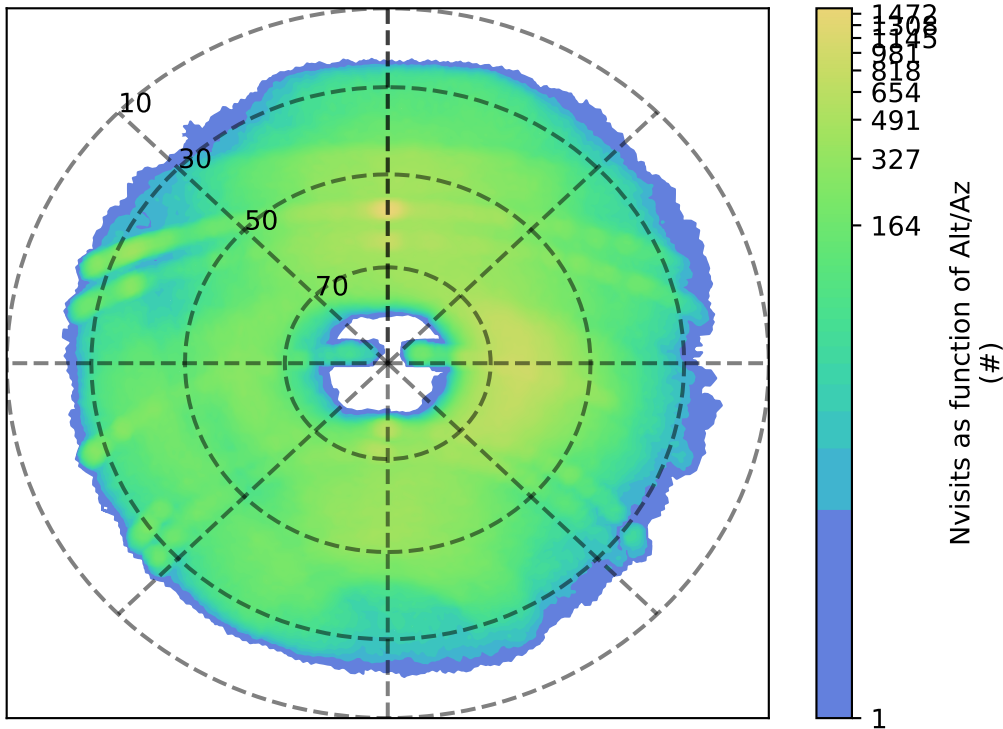
lmc_filter_balance_v3.4_10yrs g: Nvisits as function of Alt/Az
