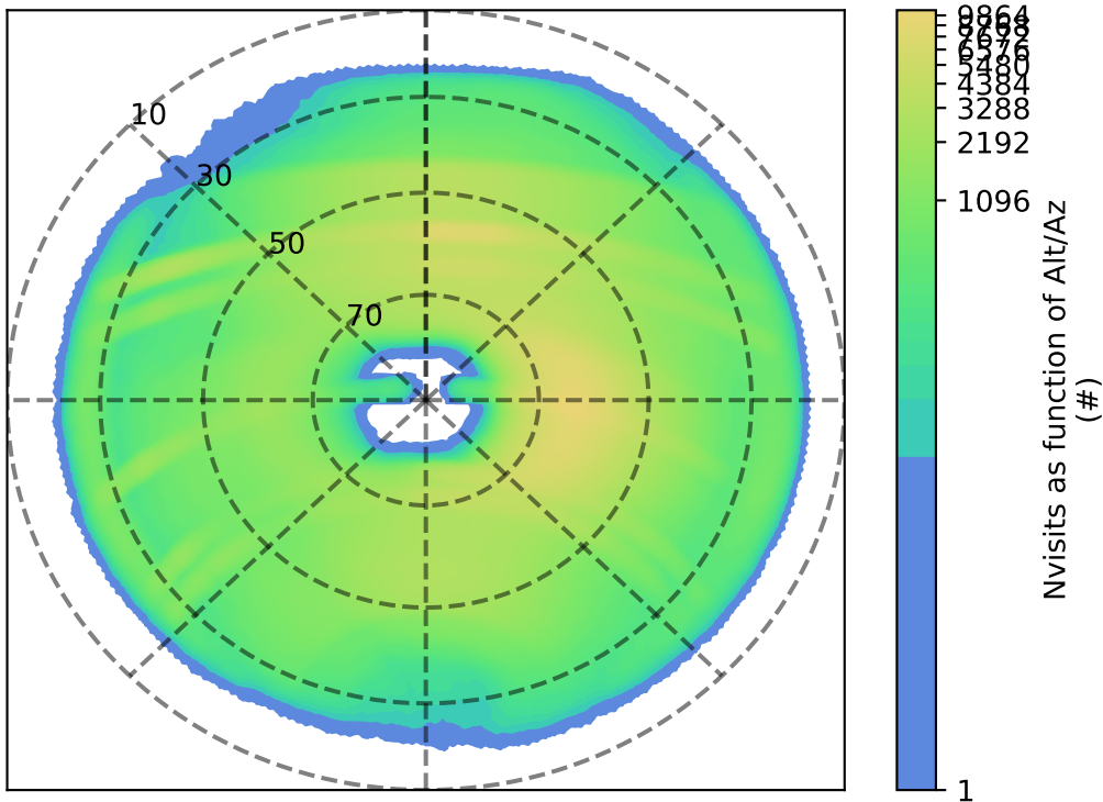
lmc_filter_balance_v3.4_10yrs : Nvisits as function of Alt/Az
