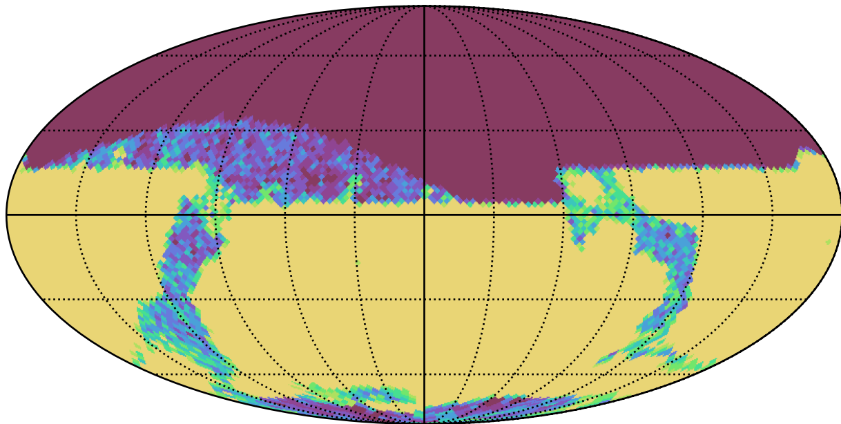
lmc_filter_balance_v3.4_10yrs z and night < 365: N year 1
