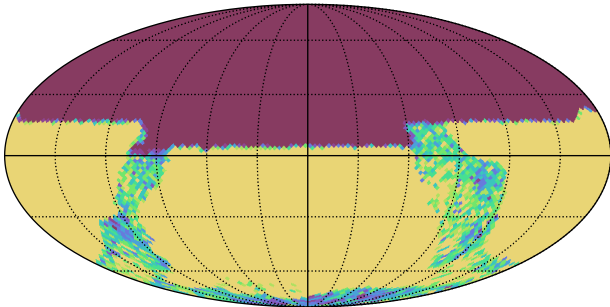
lmc_filter_balance_v3.4_10yrs y and night < 365: N year 1
