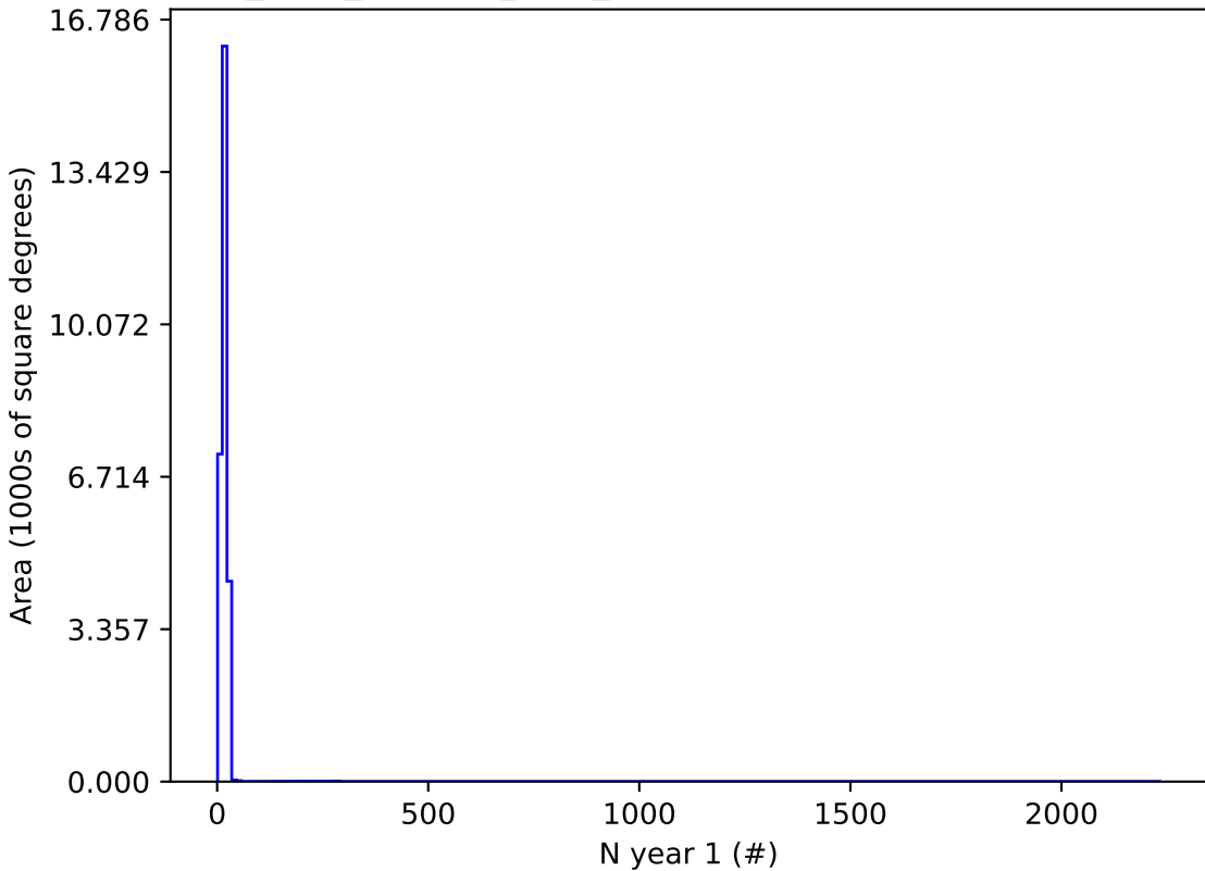
Imc_filter_balance_v3.4_10yrs i and night < 365: N year 1
