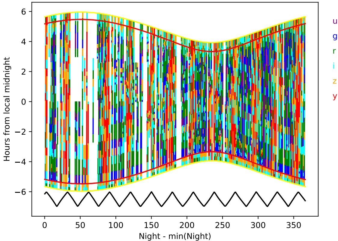
Imc_filter_balance_v3.4_10yrs year 9-10: Hourglass
