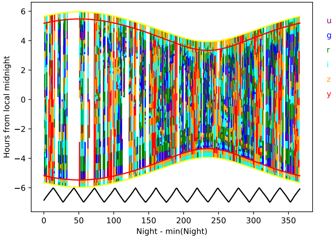
lmc_filter_balance_v3.4_10yrs year 8-9: Hourglass
