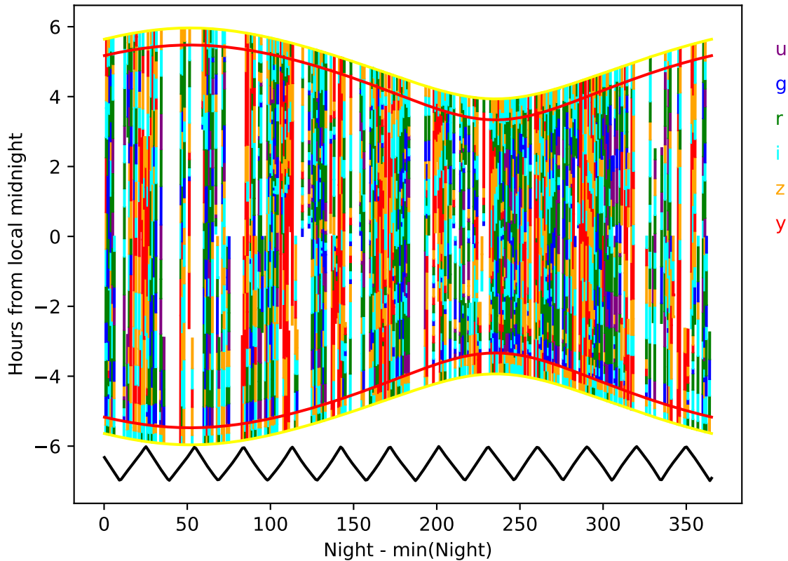
lmc_filter_balance_v3.4_10yrs year 7-8: Hourglass
