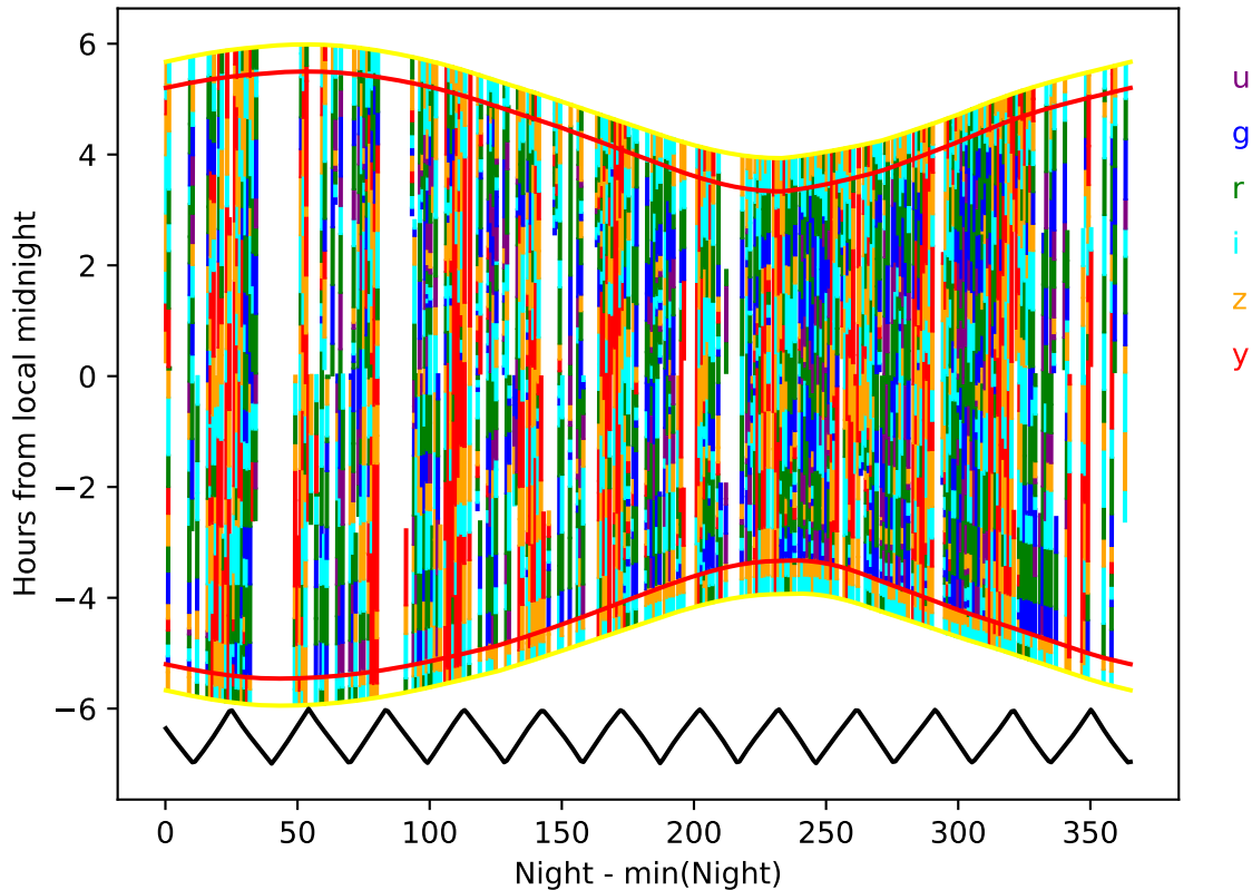
lmc_filter_balance_v3.4_10yrs year 4-5: Hourglass
