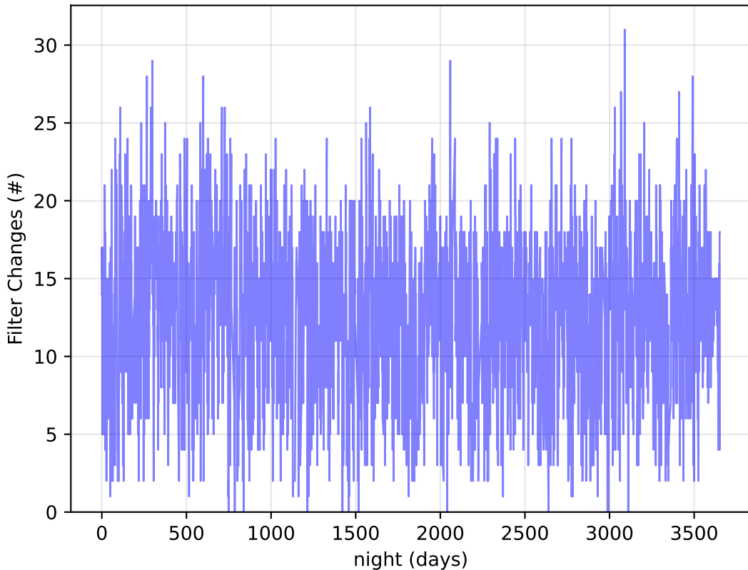
Imc_filter_balance_v3.4_10yrs : Filter Changes
