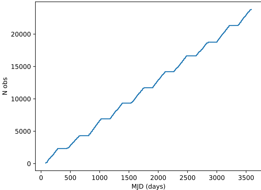
lmc_filter_balance_v3.4_10yrs note like DD:XMM_LSS%: Cumulative
