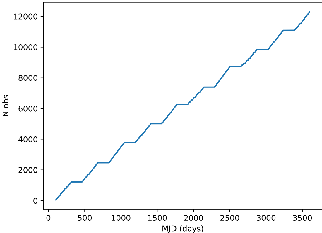
Imc_filter_balance_v3.4_10yrs note like DD:EDFS_b%: Cumulative
