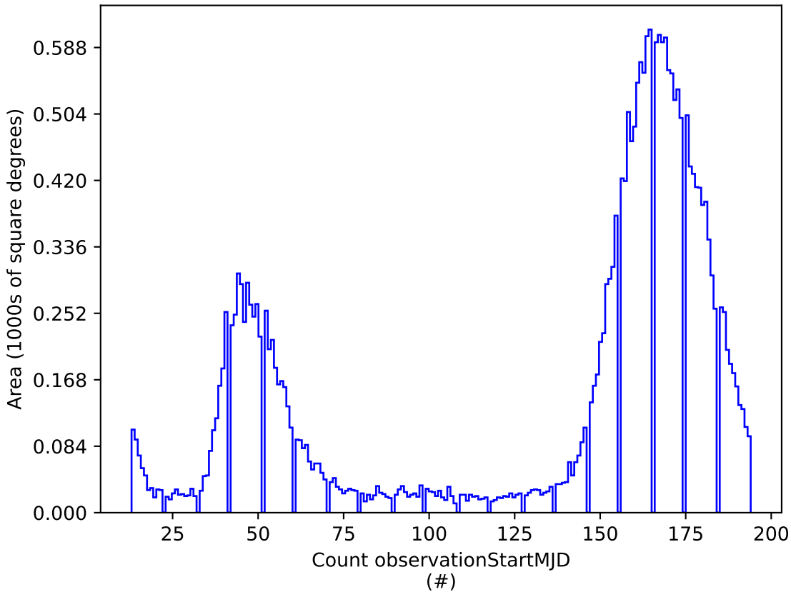
Imc_filter_balance_v3.4_10yrs z: Count observationStartMJD
