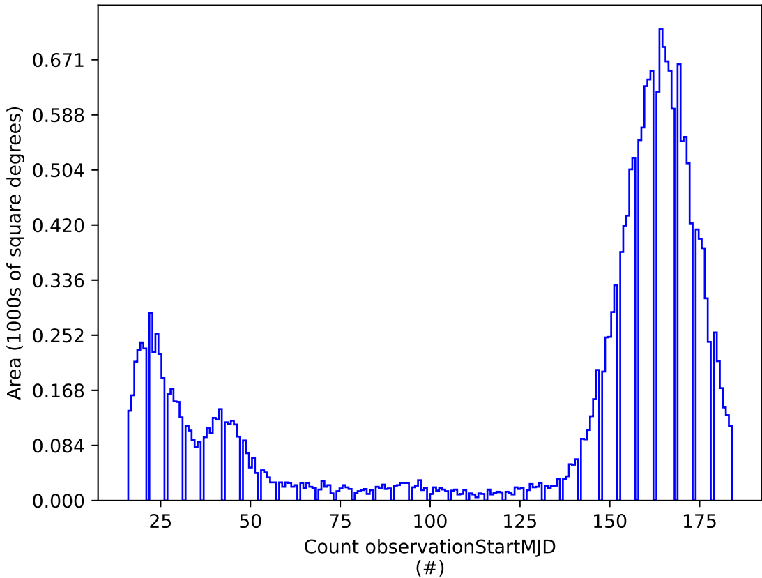
lmc_filter_balance_v3.4_10yrs y: Count observationStartMJD
