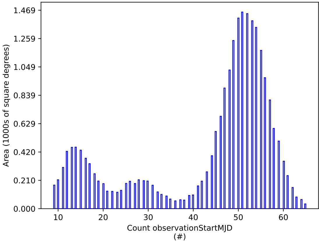
Imc_filter_balance_v3.4_10yrs u: Count observationStartMJD
