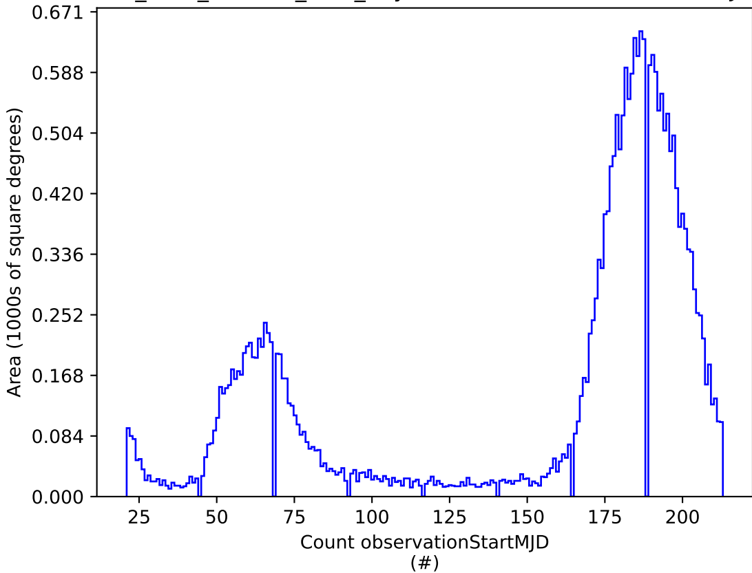
lmc_filter_balance_v3.4_10yrs i: Count observationStartMJD
