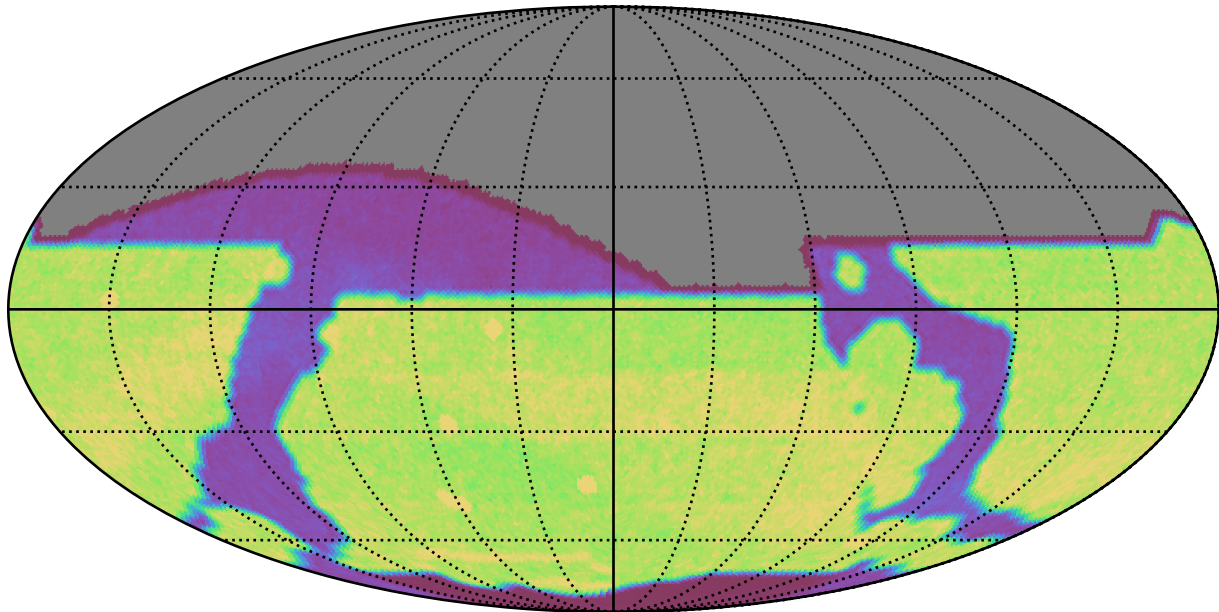
lmc_filter_balance_v3.4_10yrs : Count observationStartMJD
