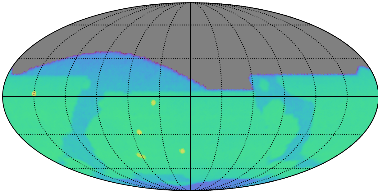
lmc_filter_balance_v3.4_10yrs z: CoaddM5
