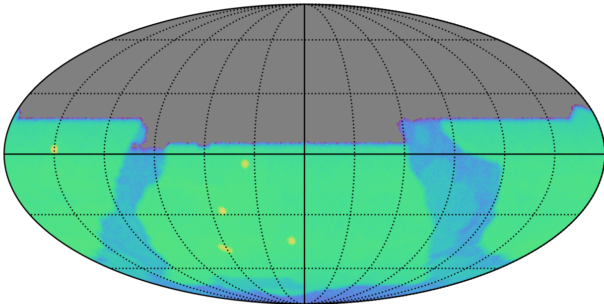
lmc_filter_balance_v3.4_10yrs y: CoaddM5
