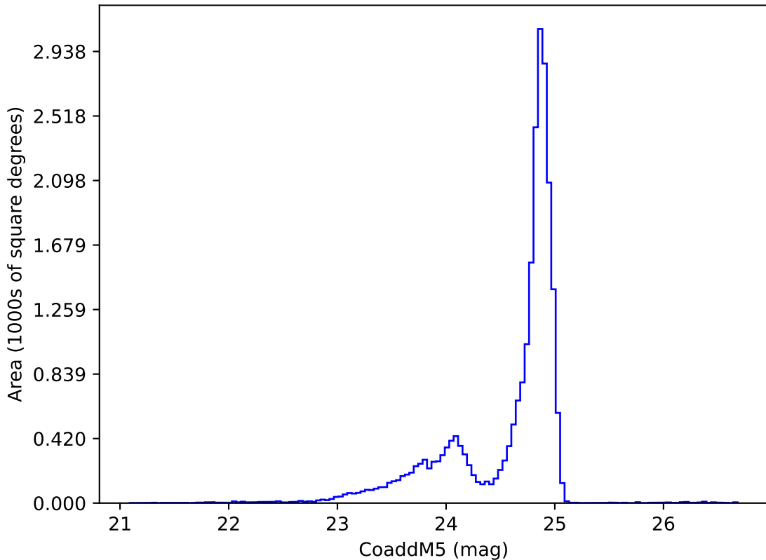
lmc_filter_balance_v3.4_10yrs y: CoaddM5
