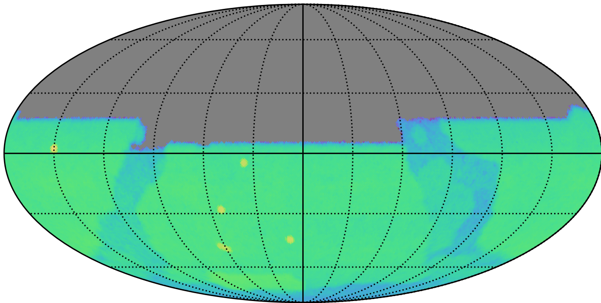
lmc_filter_balance_v3.4_10yrs u: CoaddM5
