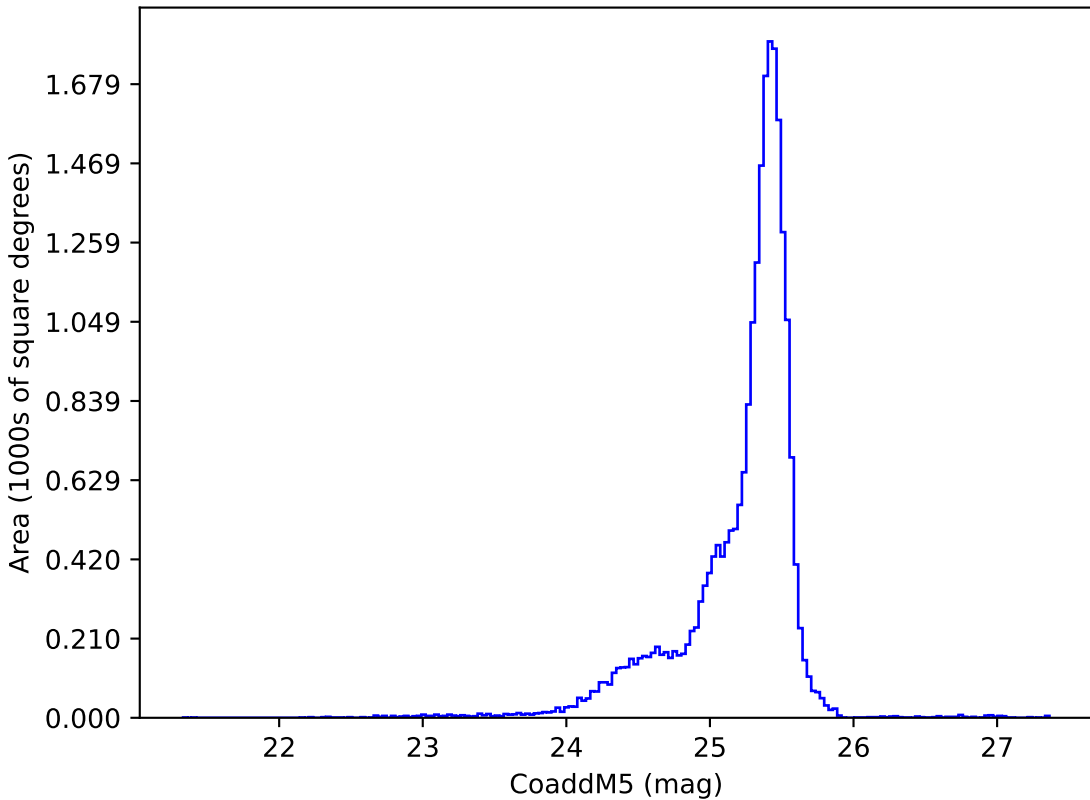
lmc_filter_balance_v3.4_10yrs u: CoaddM5
