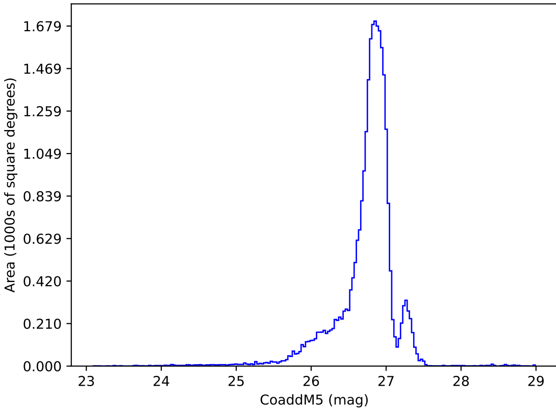
Imc_filter_balance_v3.4_10yrs g: CoaddM5
