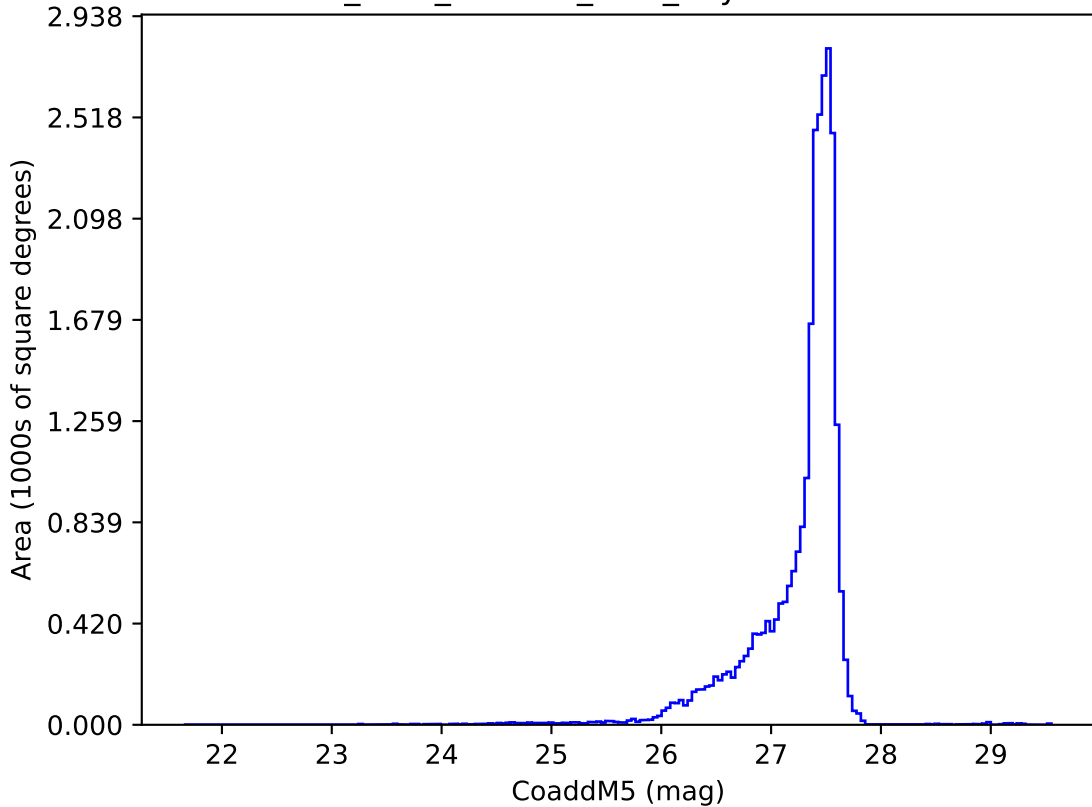
Imc_filter_balance_v3.4_10yrs : CoaddM5
