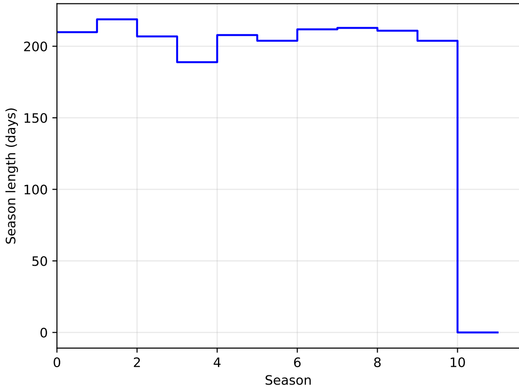
Imc_filter_balance_v3.4_10yrs DD:ELAISS1 all bands: SeasonLength
