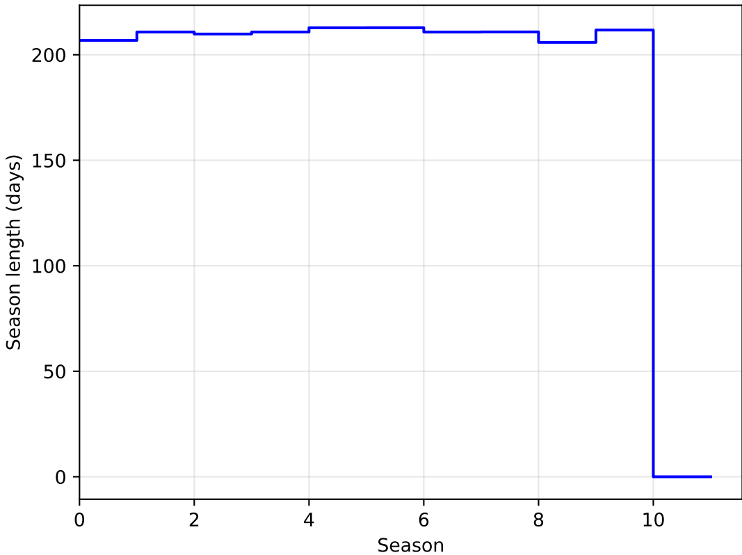
Imc_filter_balance_v3.4_10yrs DD:EDFS all bands: SeasonLength
