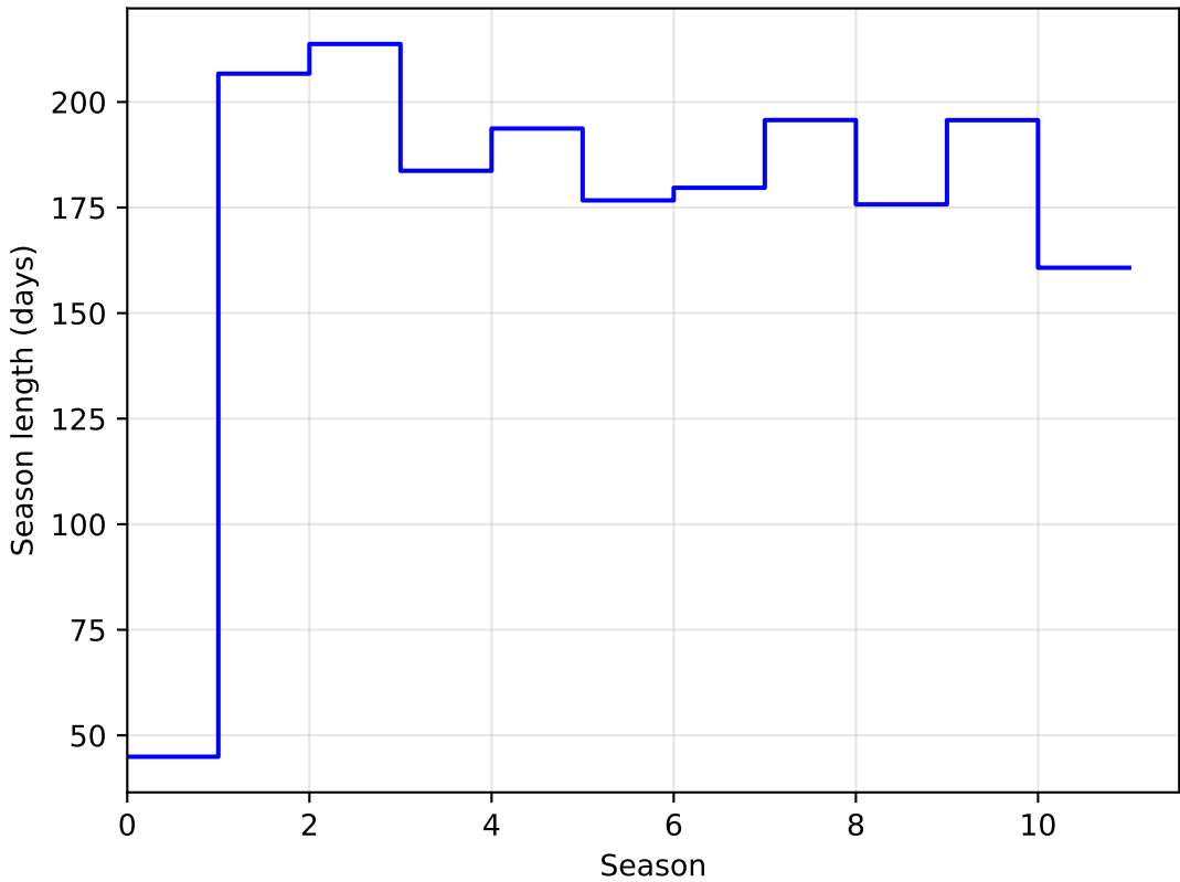
Imc_filter_balance_v3.4_10yrs DD: COSMOS all bands: SeasonLength
