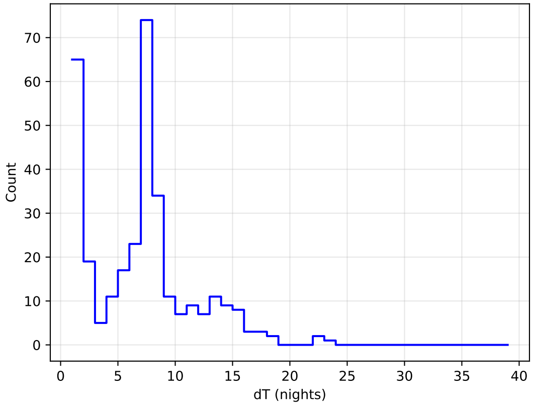
Imc_filter_balance_v3.4_10yrs all bands: DD:XMM_LSS Delta Nights Histogram
