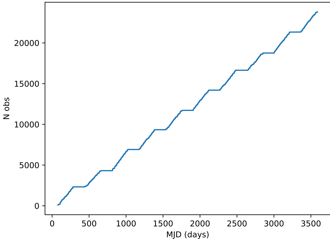
Imc_filter_balance_v3.4_10yrs all bands: DD:XMM_LSS Cumulative NVisits
