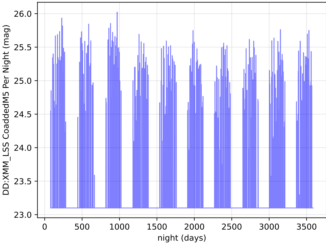
Imc_filter_balance_v3.4_10yrs i band: DD:XMM_LSS CoaddedM5 Per Night
