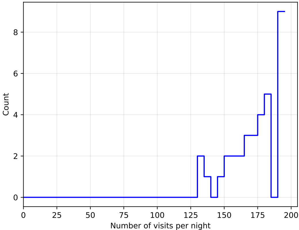
Imc_filter_balance_v3.4_10yrs all bands: DD:WFD NVisitsPerNight
