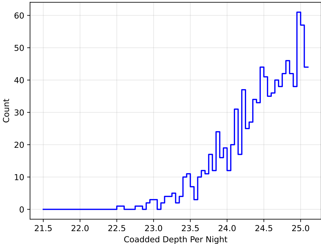
Imc_filter_balance_v3.4_10yrs y band: DD:WFD CoaddM5PerNight
