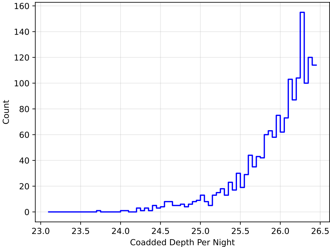
Imc_filter_balance_v3.4_10yrs i band: DD:WFD CoaddM5PerNight
