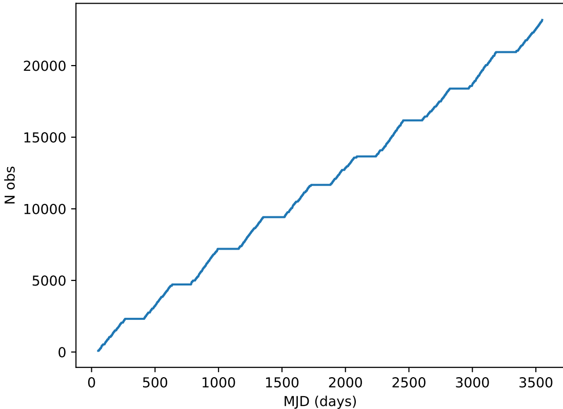
Imc_filter_balance_v3.4_10yrs all bands: DD:ELAISS1 Cumulative NVisits
