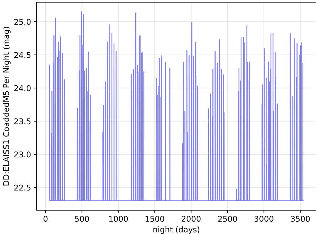
Imc_filter_balance_v3.4_10yrs u band: DD:ELAISS1 CoaddedM5 Per Night
