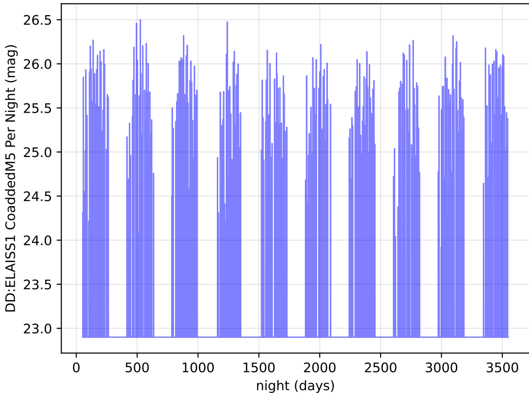
Imc_filter_balance_v3.4_10yrs r band: DD:ELAISS1 CoaddedM5 Per Night
