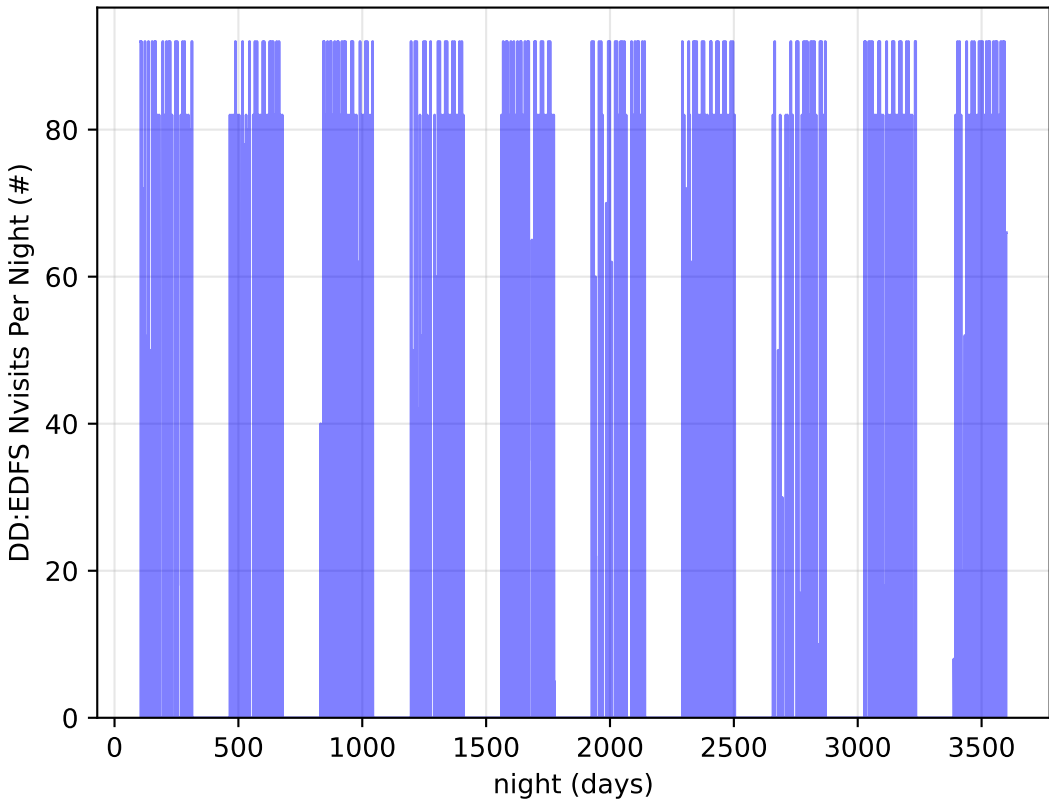
Imc_filter_balance_v3.4_10yrs all bands: DD:EDFS Nvisits Per Night
